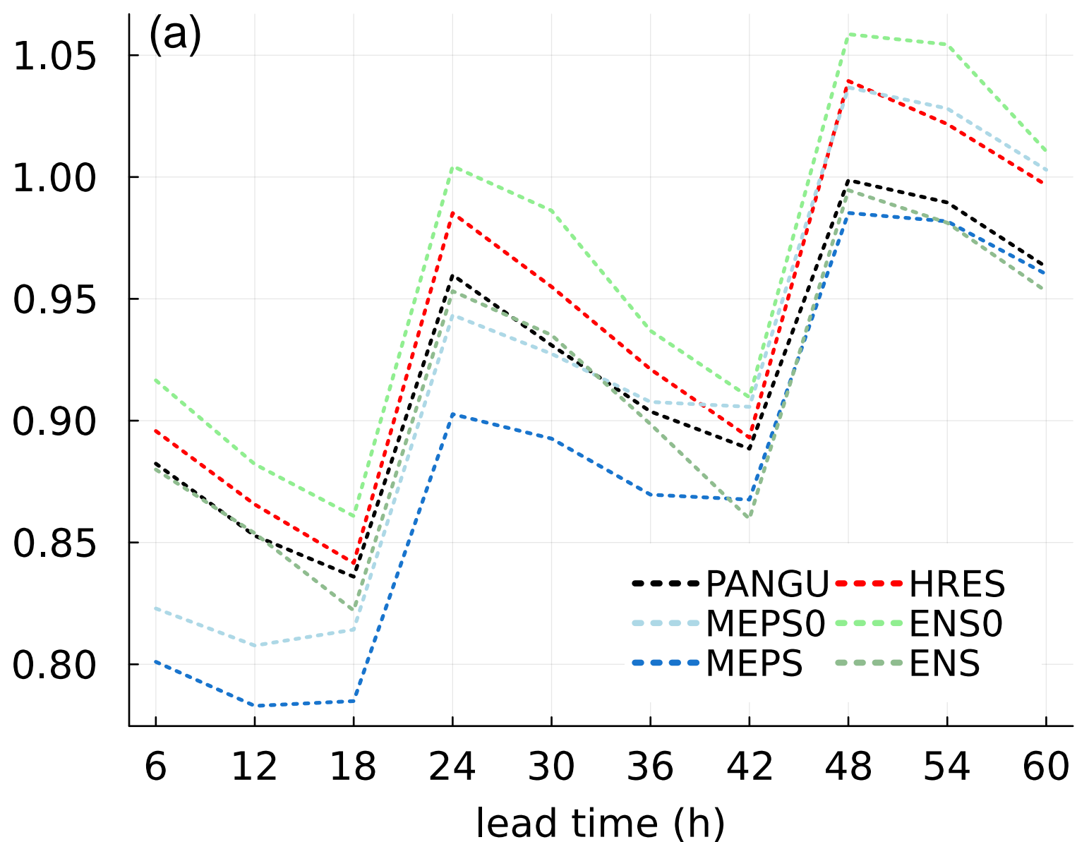
continuous ranked probability score (K)
