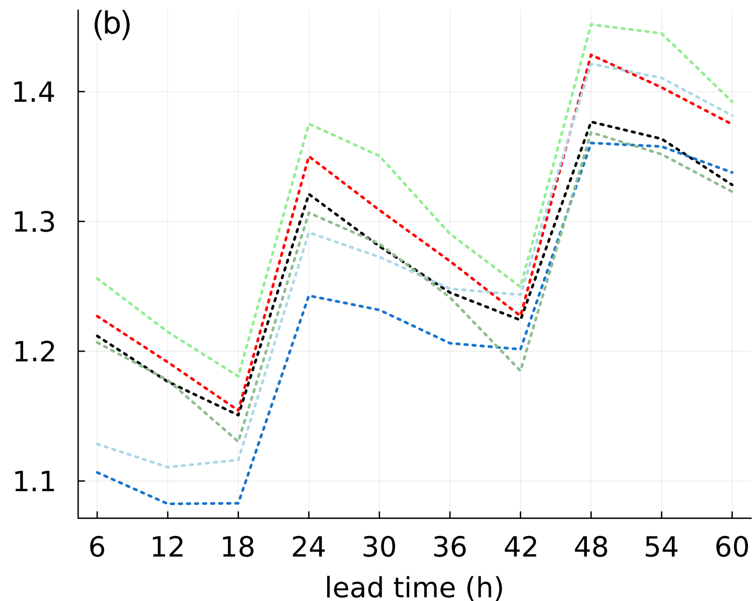
mean absolute error (K)
