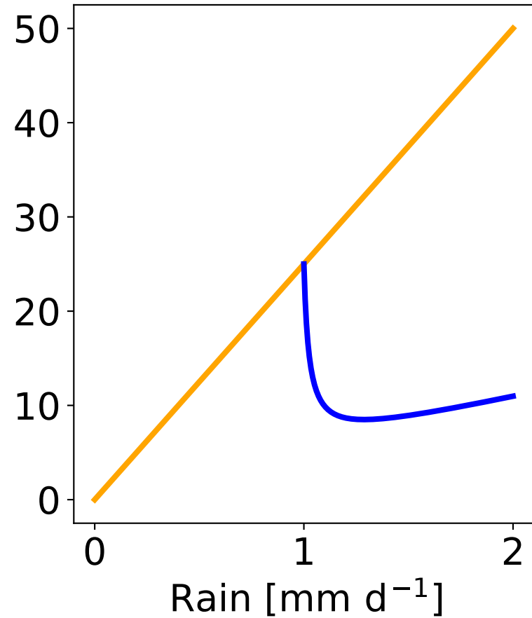
(c) Surface water [mm]
