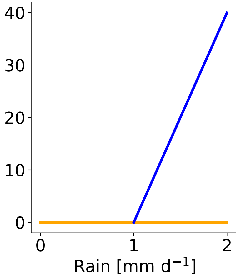
(a) Biomass [ \text{g m}^{-2} ]
