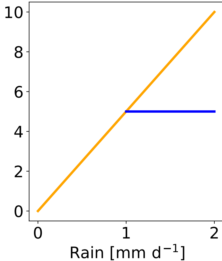
(b) Soil water [mm]
