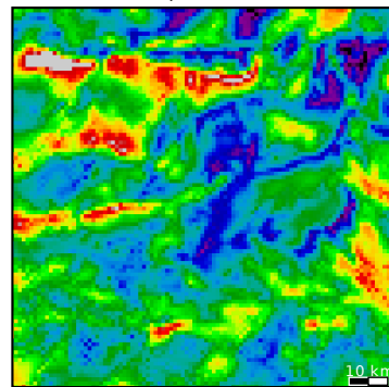
(f) Mean wind speed (HR) ( \text{m s}^{-1} )
