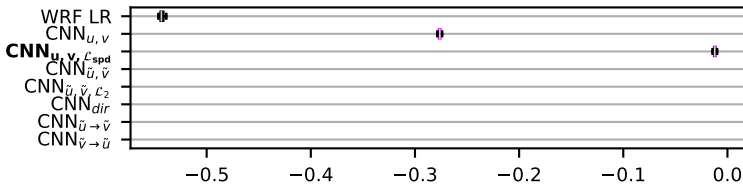
(c) Wind direction MAE ( ^{\circ} )
