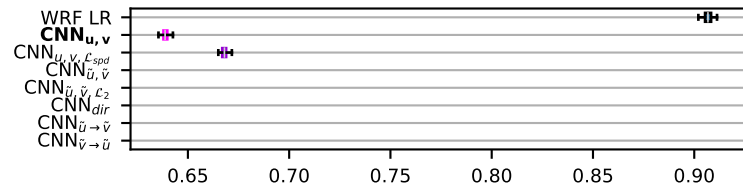
(e) u-component MBE ( \text{m s}^{-1} )
