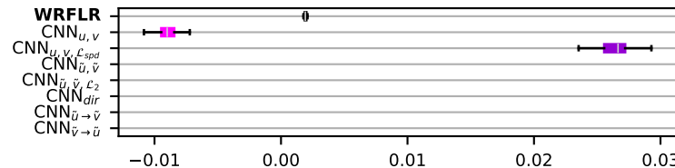
(f) v-component MAE ( \text{m s}^{-1} )
