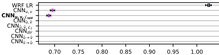
(b) Wind speed MBE ( \text{m s}^{-1} )
