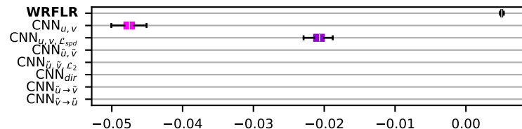
(g) v-component MBE ( \text{m s}^{-1} )
