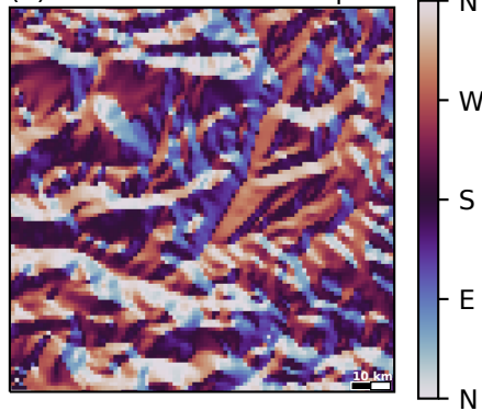
(b) Orientation of the slope
