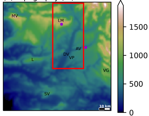
(a) Topography (m)
