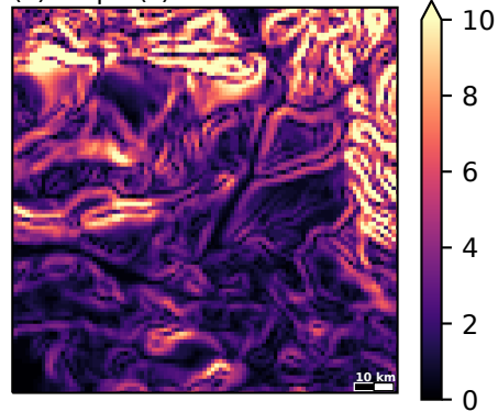
(c) Slope ( ^{\circ} )
