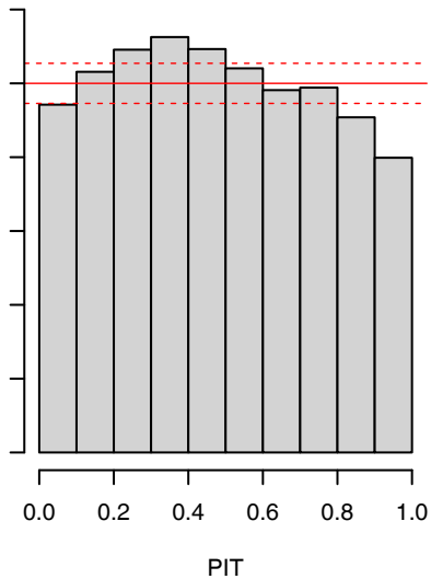
Distributional forest
