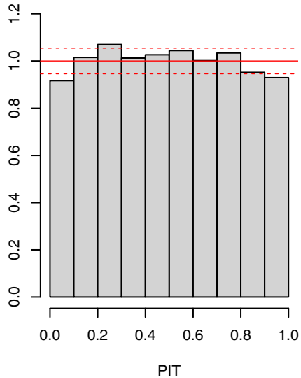
MOS forest
