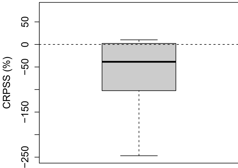
(c) RAINR=0, 1 SNOWR>0, obs>1cm [8.9%]
