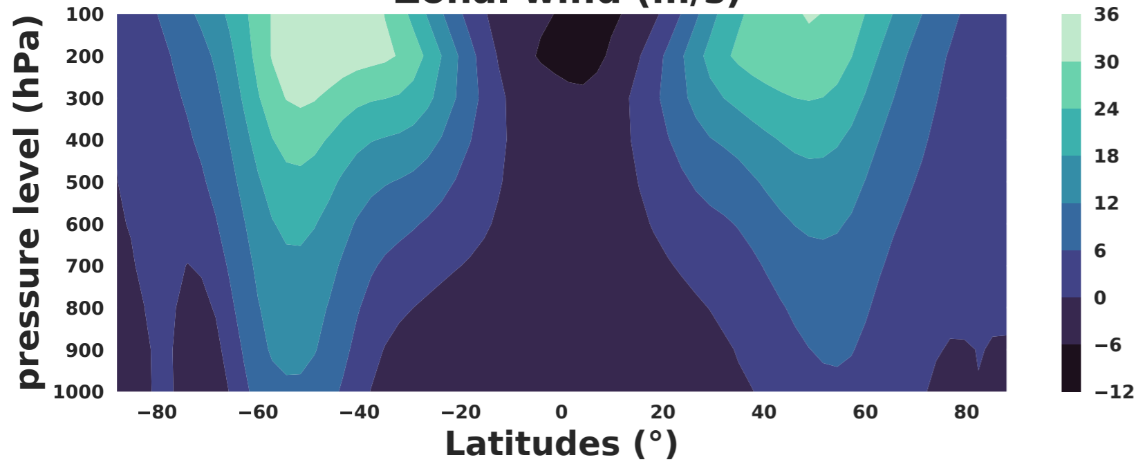
(c) Zonal wind (m/s)
