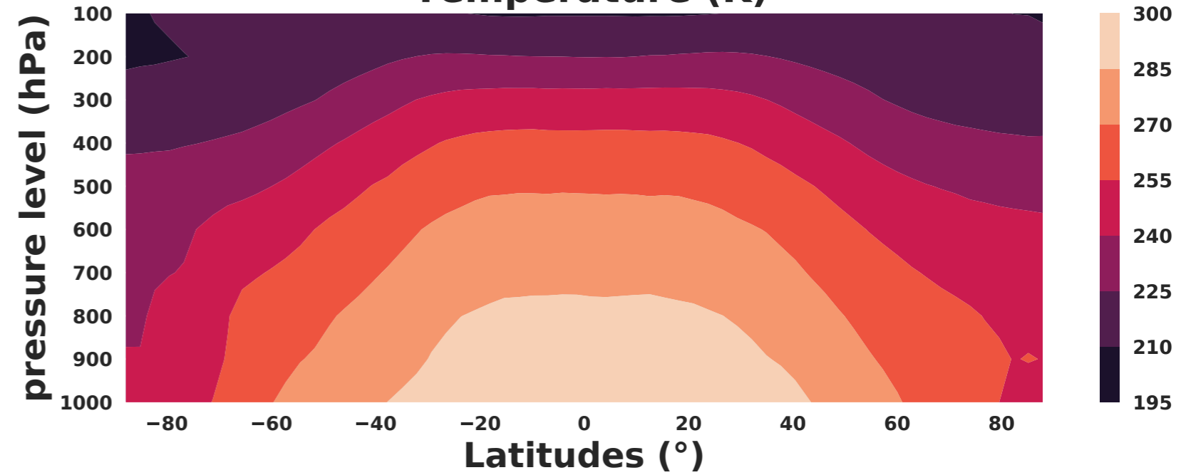
(b) Temperature (K)
