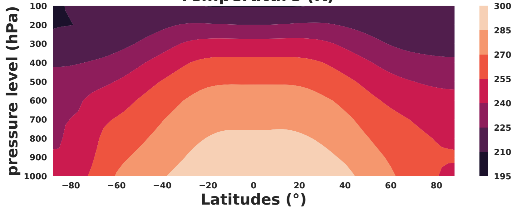
(a) Temperature (K)
