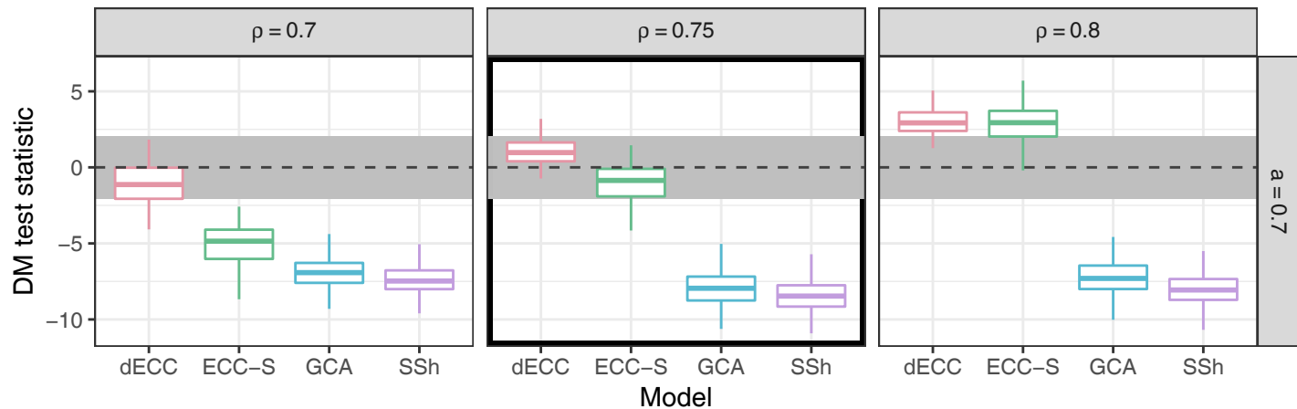
(b) Variogram score, \sigma = 1, \rho_0 = 0.75
