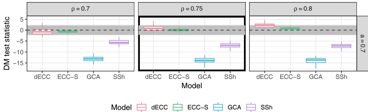
(a) Energy score, \sigma = 1, \rho_0 = 0.75
