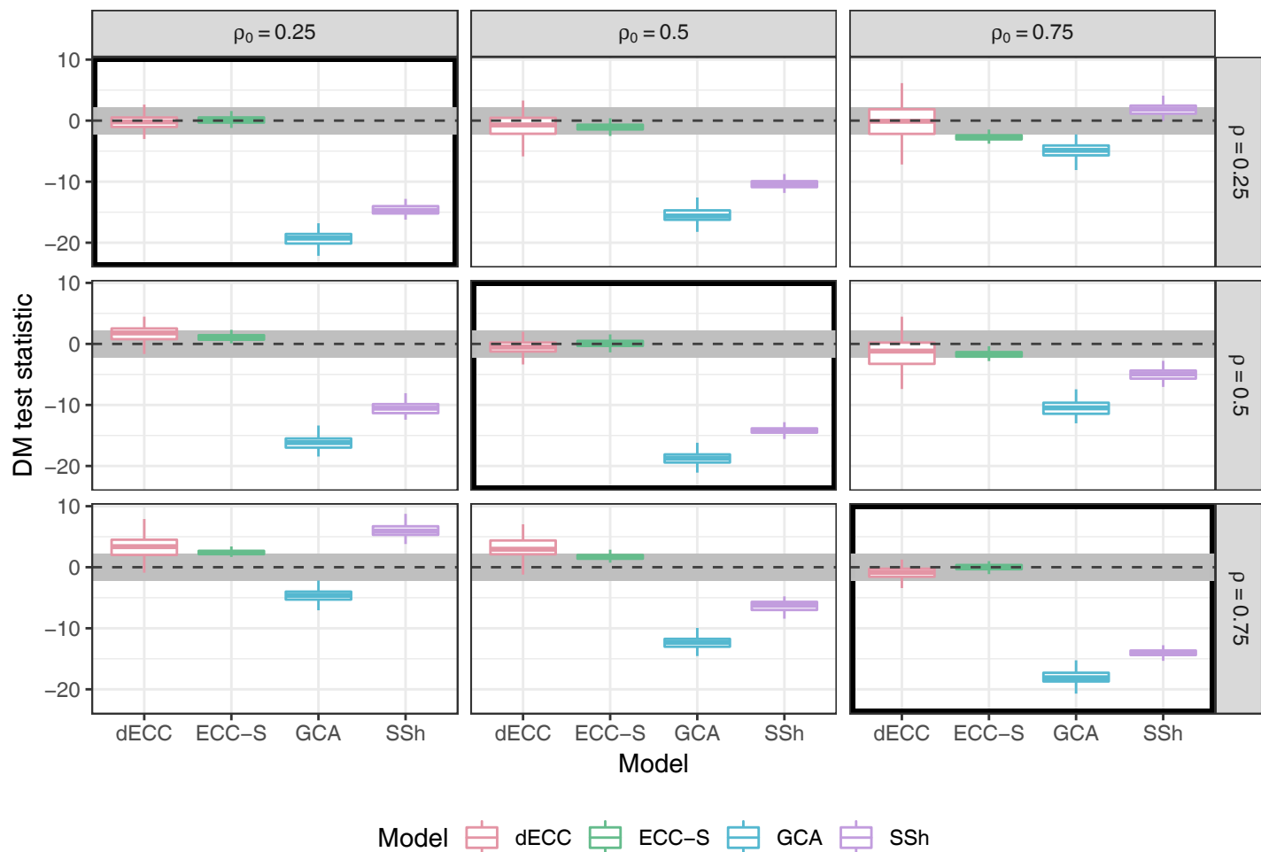
(a) Energy score, \sigma = 1
