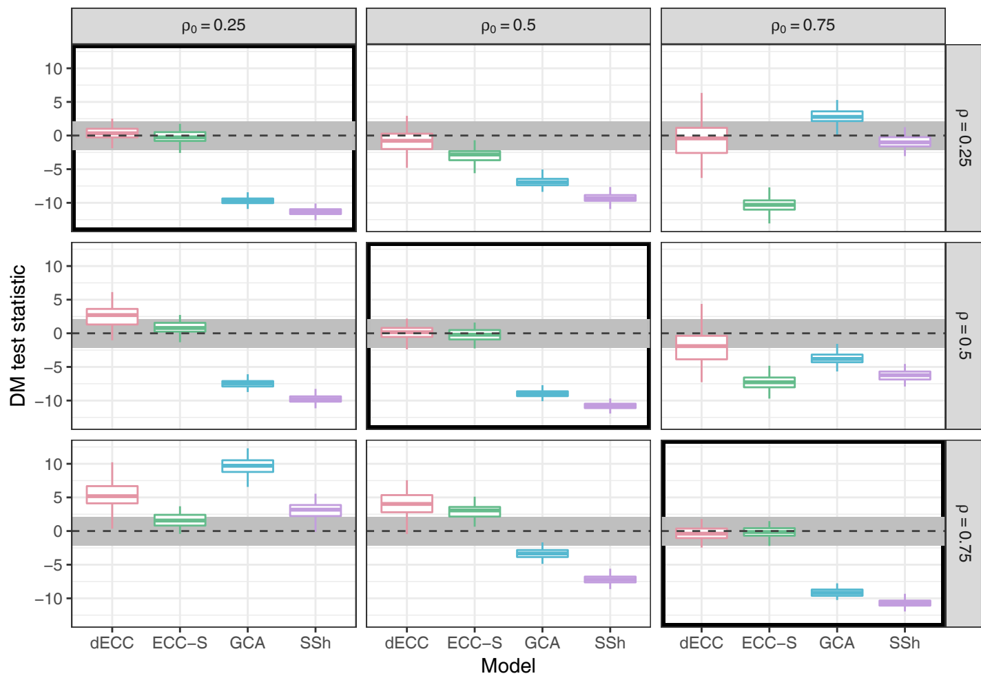
(b) Variogram score, \sigma = 1
