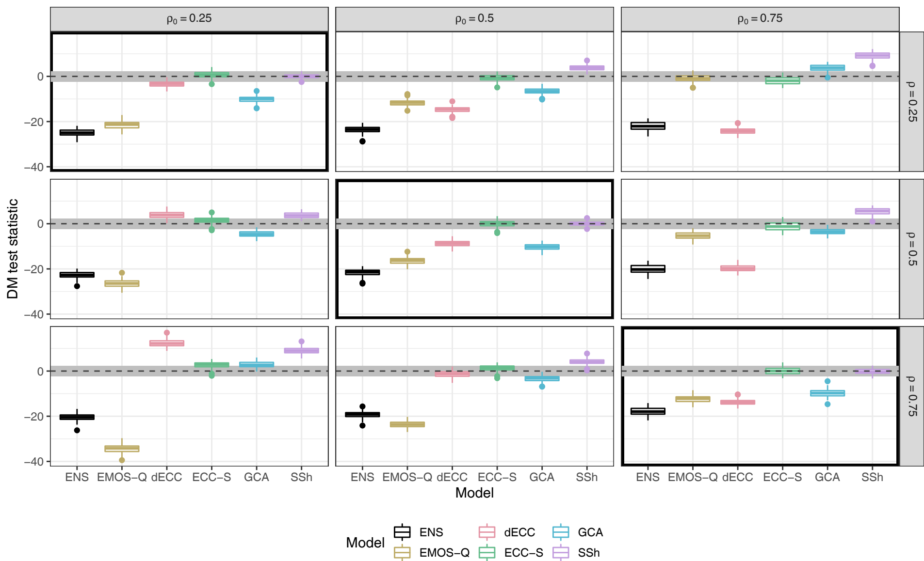
(a) Energy score, m = 50, \mu_0 = 0, \sigma_0 = 1, \xi_0 = -0.1, \mu = 0, \sigma = 2, \xi = 0
