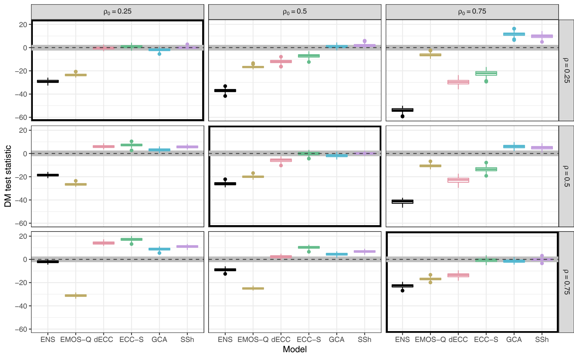
(b) Variogram score, m = 50, \mu_0 = 0, \sigma_0 = 1, \xi_0 = -0.1, \mu = 0, \sigma = 2, \xi = 0
