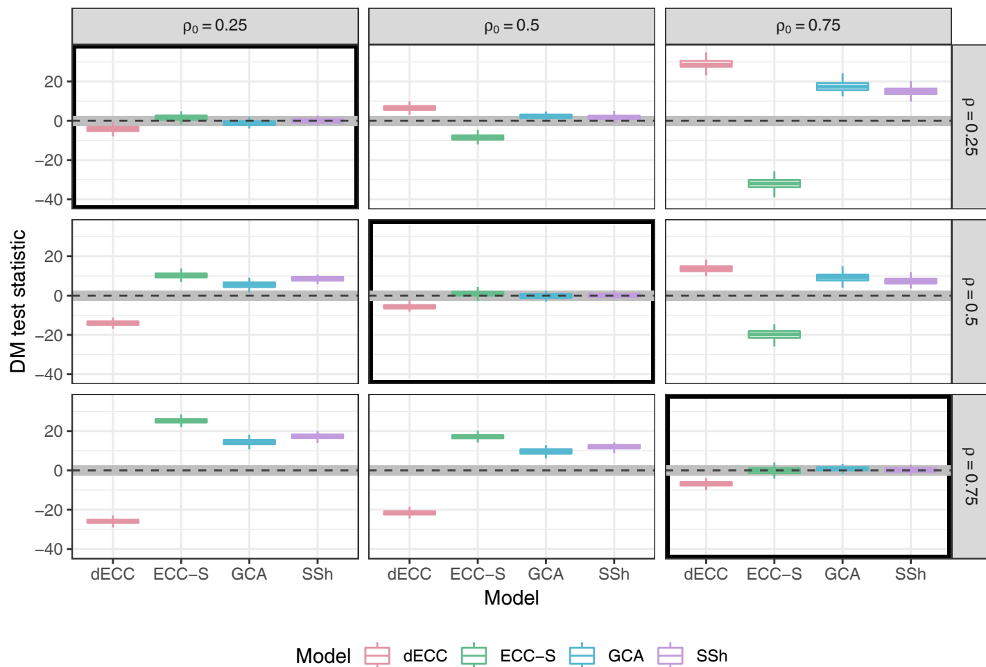
(a) Variogram score, \sigma = 0.5
