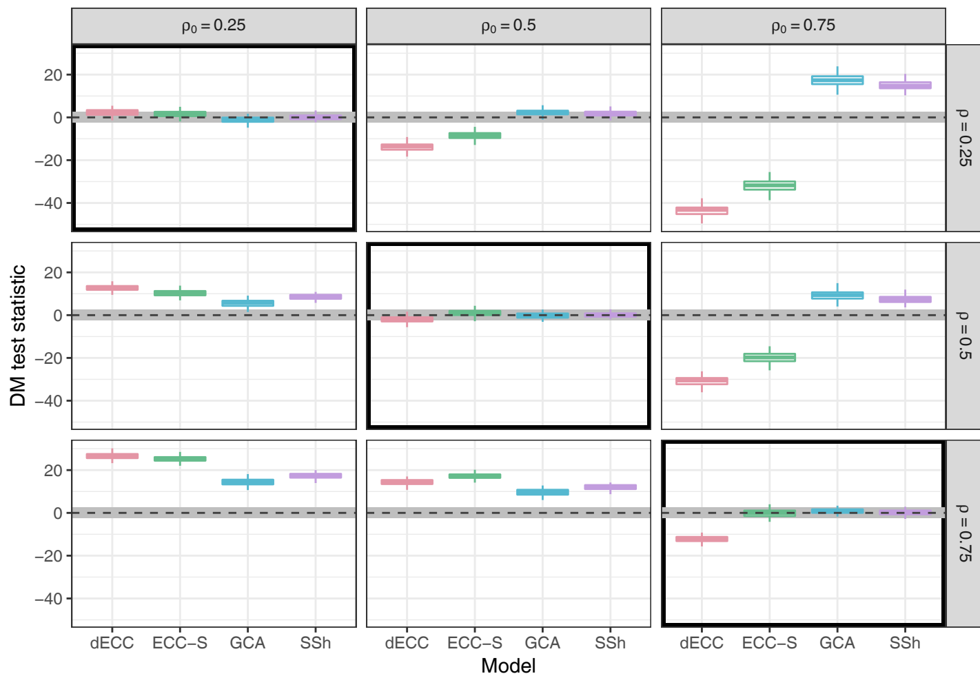
(b) Variogram score, \sigma = 2.24
