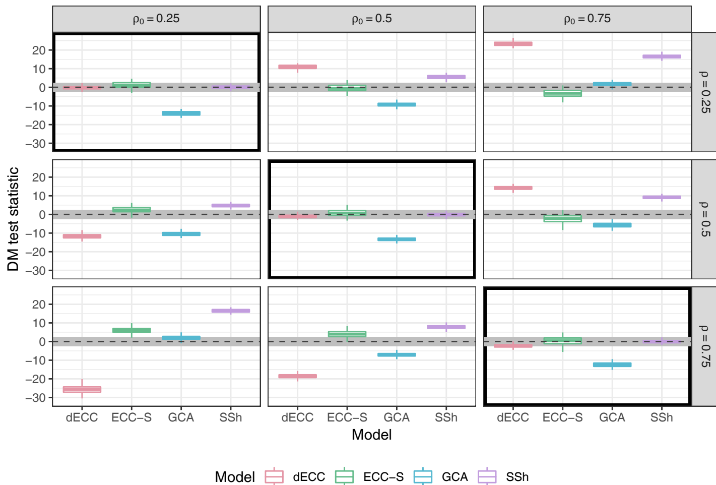
(a) Energy score, \sigma = 0.5
