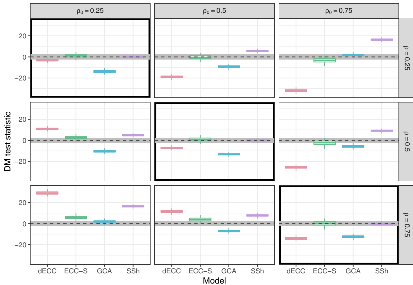
(b) Energy score, \sigma = 2.24
