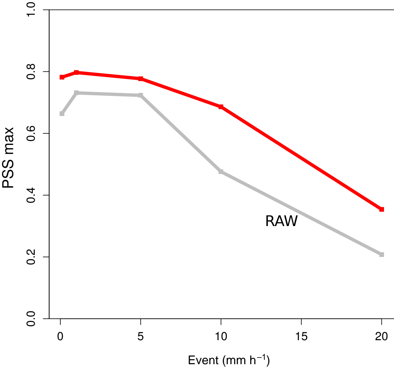
Time-averaged maximum of Peirce's Skill Score
