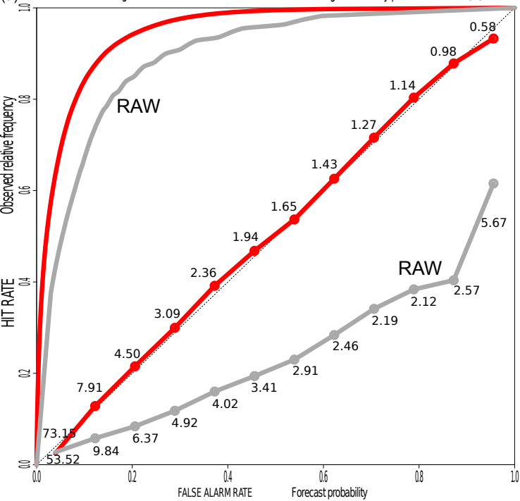
Time-averaged ROC Curve >0.1\text{mm h}^{-1} event
