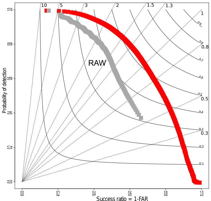
Time-averaged Roebber diagram >0.1\text{mm h}^{-1} event
