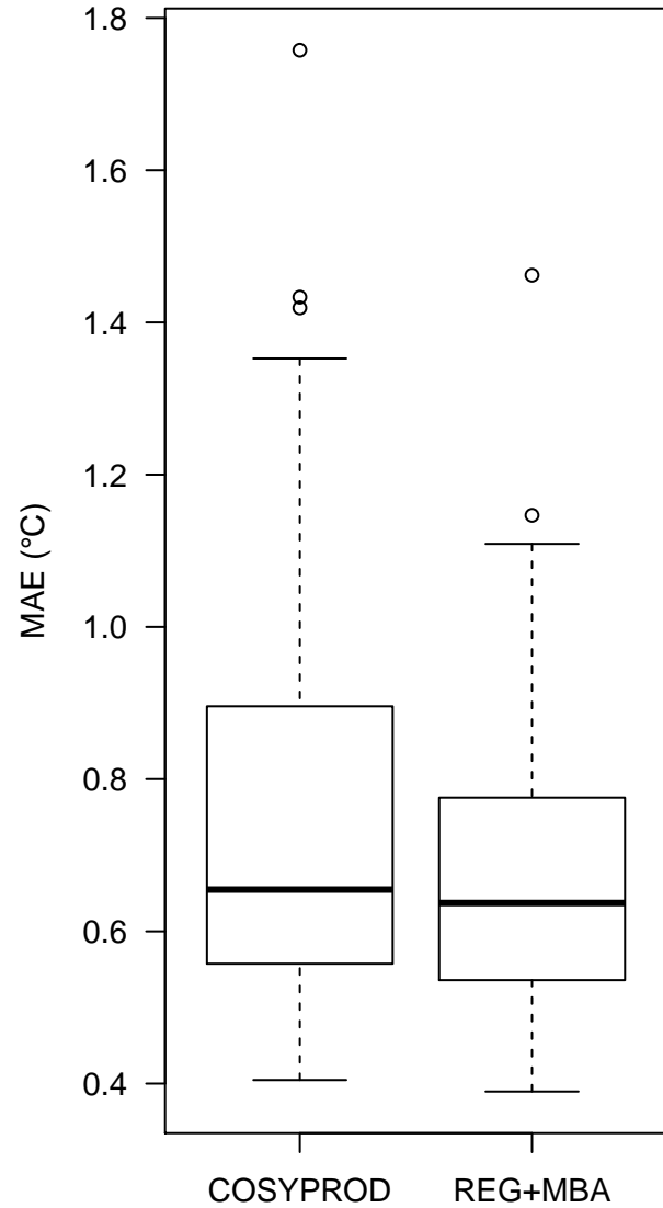
(b) MAE
