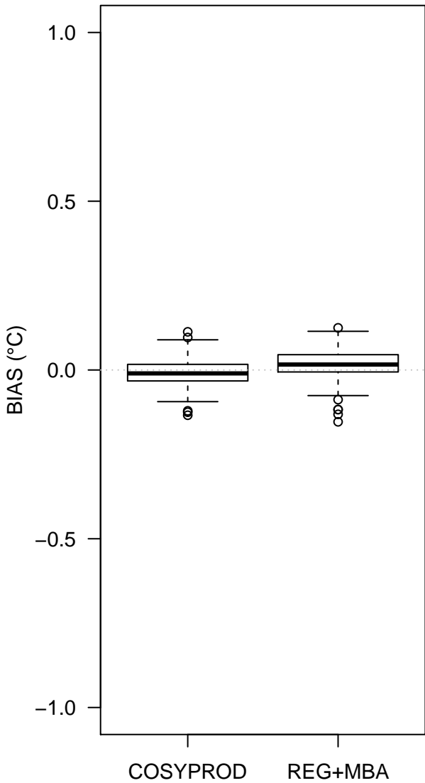
(a) BIAS
