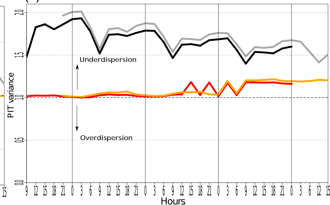
T2m PIT variance on EURW1S100 stations
