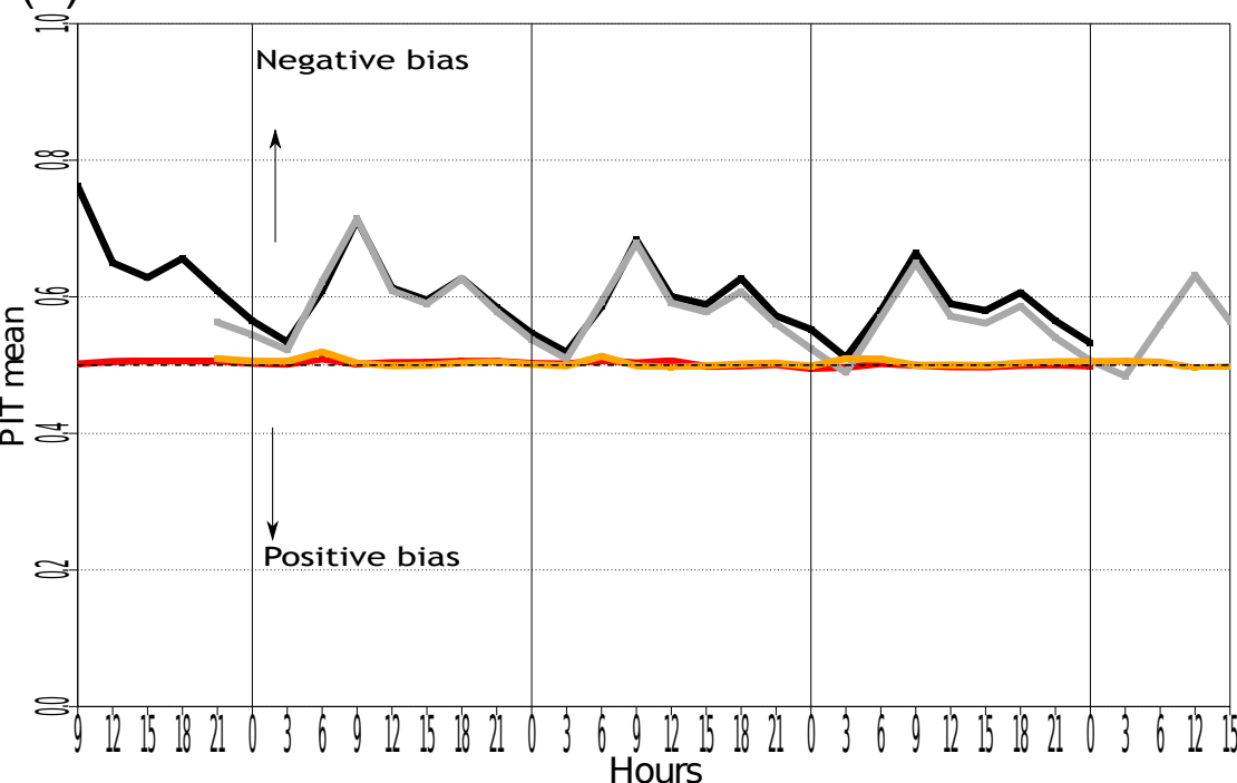
T2m PIT mean on EURW1S100 stations
