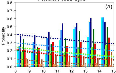
Persistent wSBL nights
