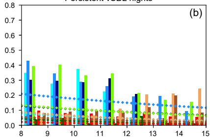
Persistent vSBL nights
