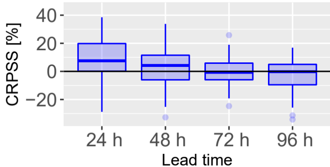
(b) Predictors for verification: Real-time forecasts
