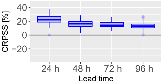
(a) Predictors for verification: Reforecasts
