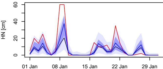
(c) + 72 h, station: 73023401, CRPSS: -0.9 %
