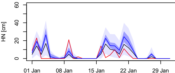
(a) + 24 h, station: 73235400 , CRPSS: 39.19 %
