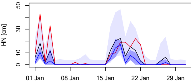
(a) + 48 h, station: 73034400, CRPSS: 31.28 %
