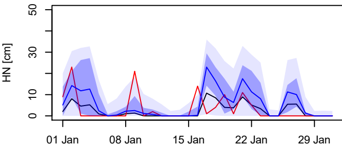
(c) + 96 h, station: 73235400, CRPSS: 29.51 %
