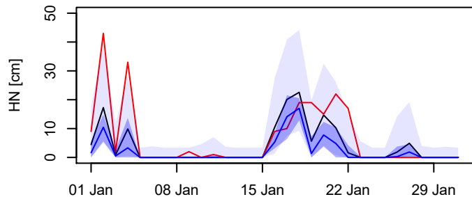
(b) + 48 h, station: 73034400, CRPSS: 28.41 %
