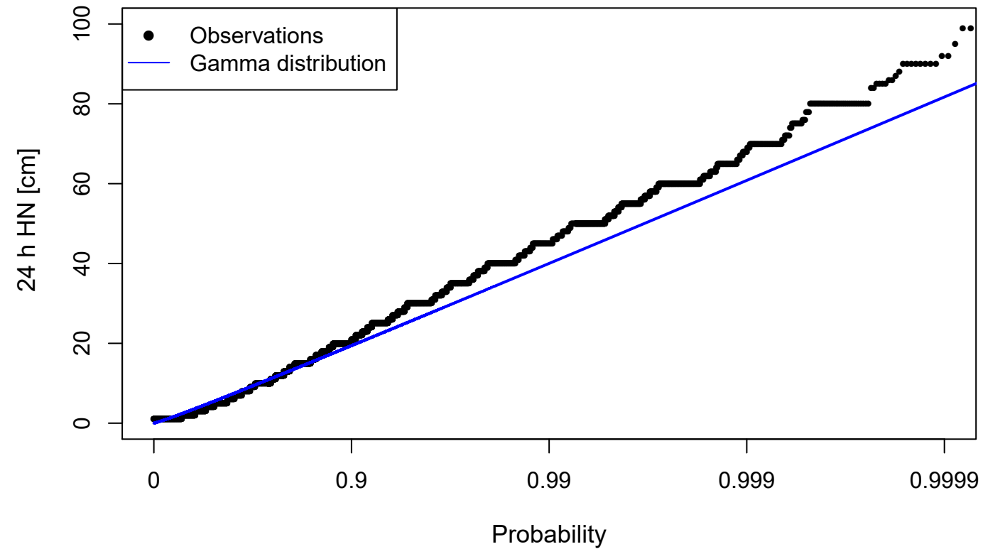
(b) Empirical CDF of HN
