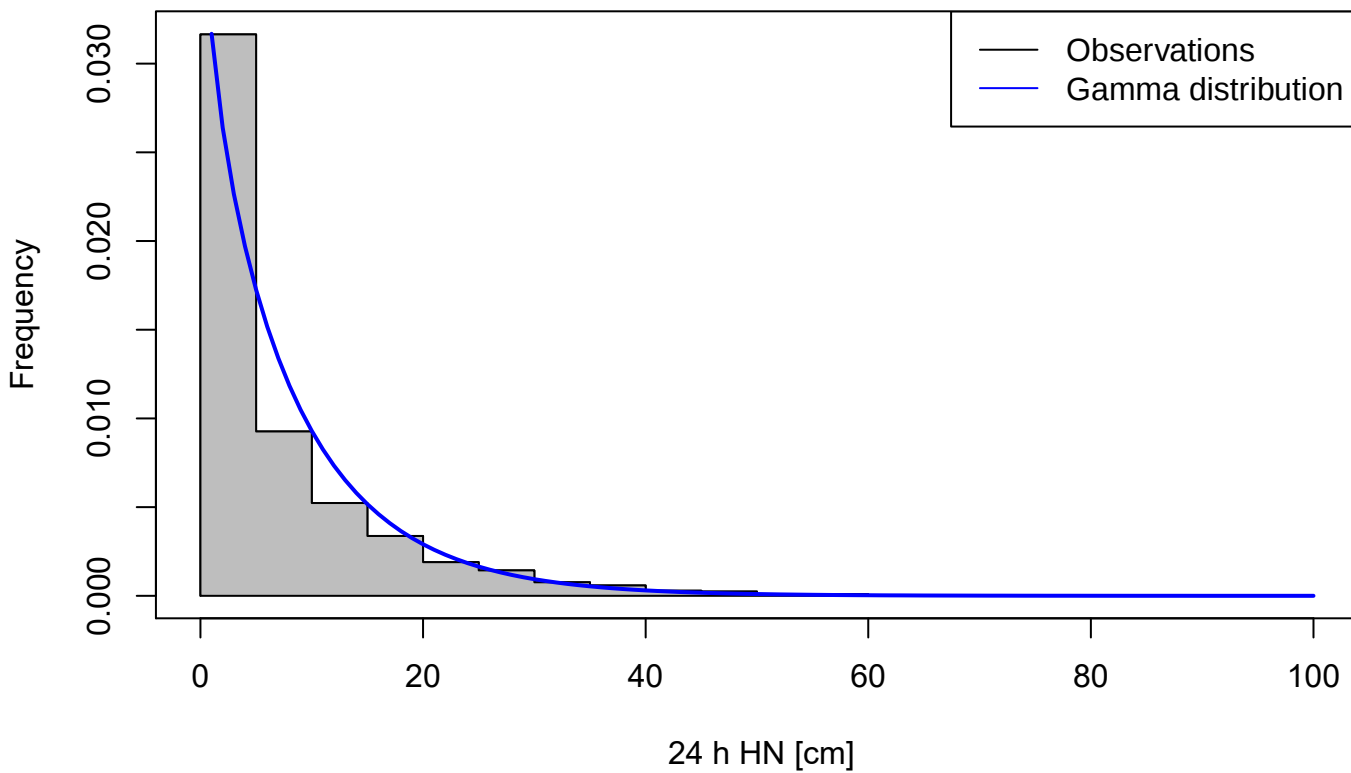
(a) Density histogram with PDFs
