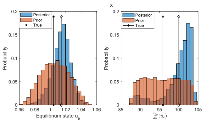
(b) Uniform prior
