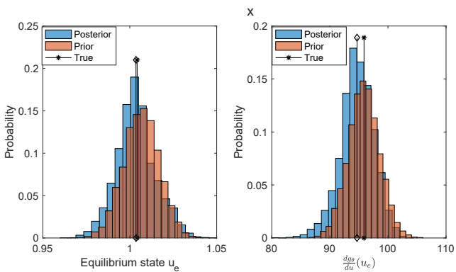
(a) Gaussian prior
