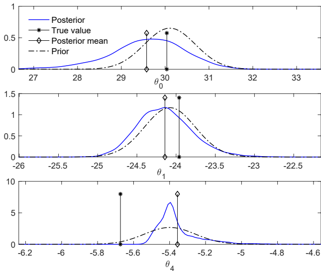
(a) Gaussian prior
