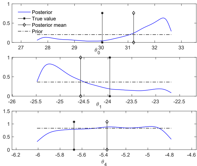
(b) Uniform prior
