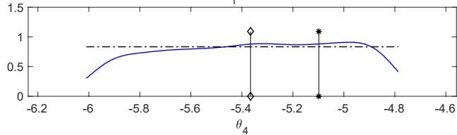
(b) Uniform prior
