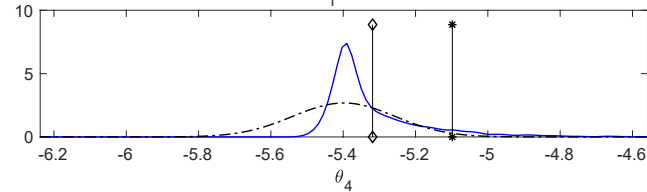
(a) Gaussian prior
