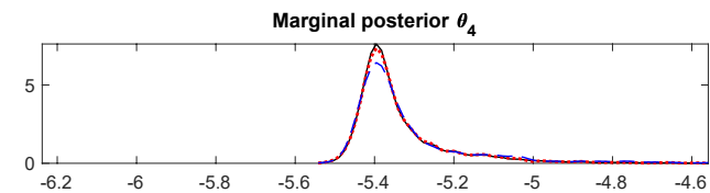
(a) Gaussian prior
