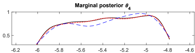
(b) Uniform prior
