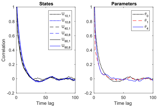
(a) Gaussian prior
