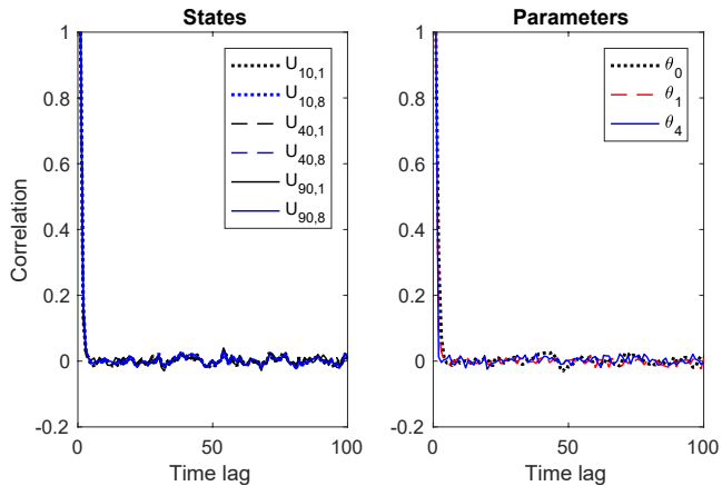
(b) Uniform prior
