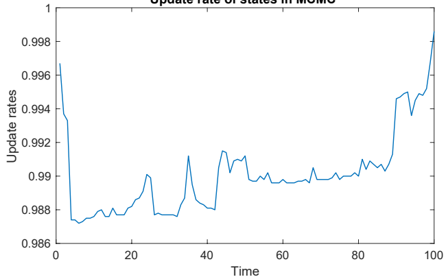
(b) Uniform prior
