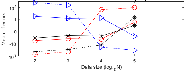
Mean of errors of MLE from true and noisy trajectories
