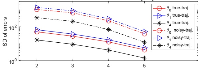
SD of errors of MLE from true and noisy trajectories
