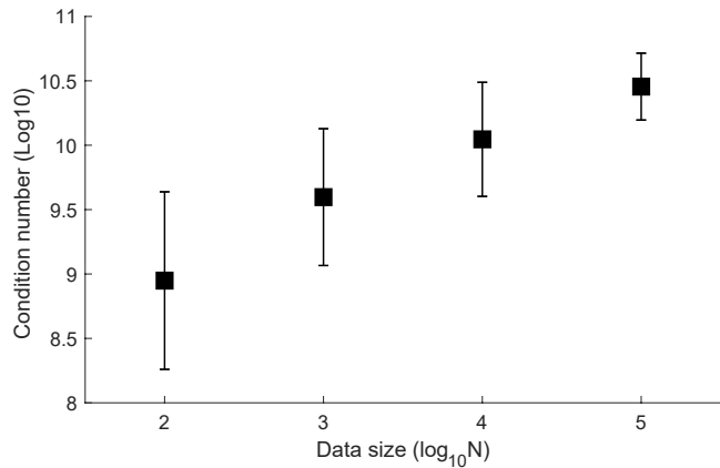
(b) Uniform prior
