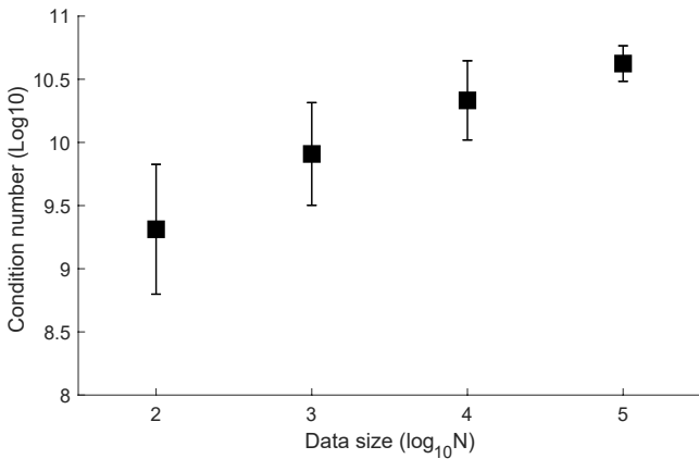
(a) Gaussian prior
