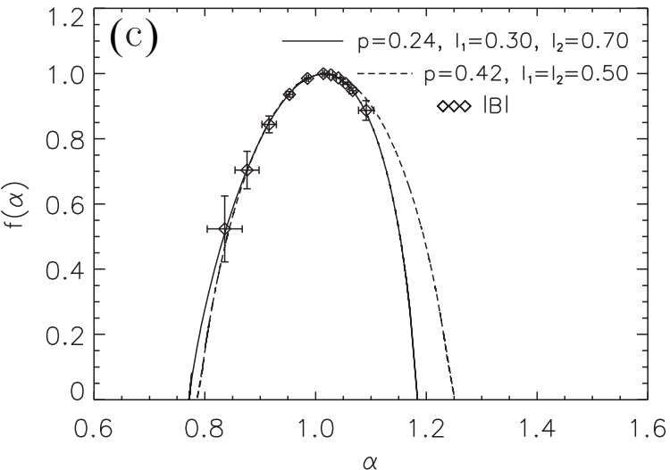
V1 2008, 1–256, R = 105–107 AU
