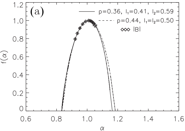
V1 2005, 1–256, R = 94–97 AU
