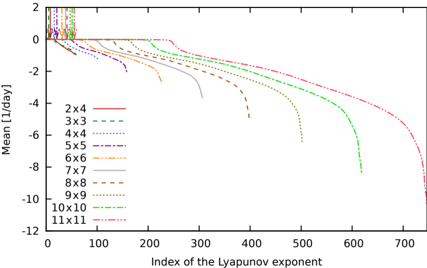
Lyapunov exponents for the dissipation x10 model configurations
