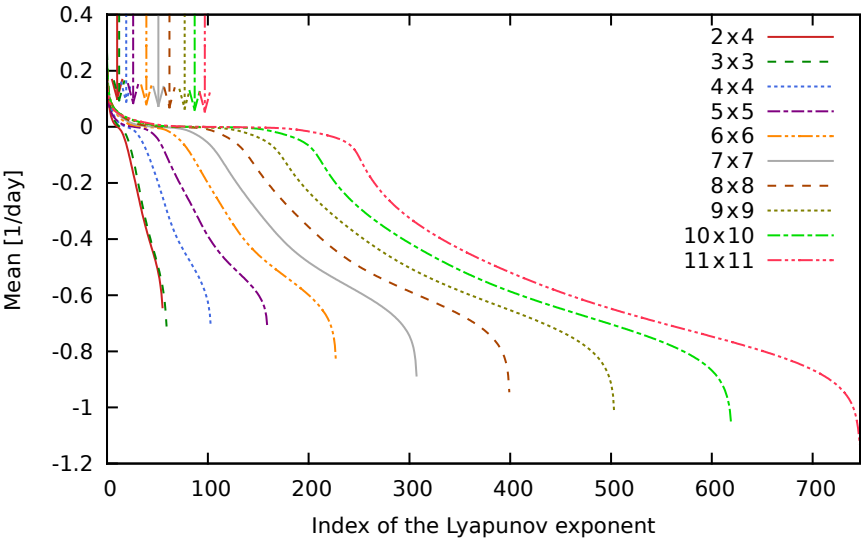
Lyapunov exponents for the dissipation model configurations
