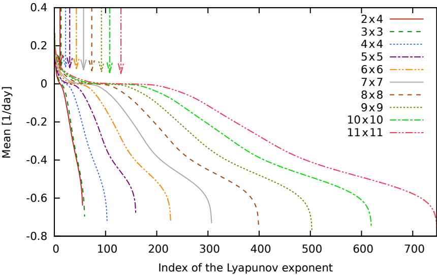
Lyapunov exponents for the nodissip model configurations
