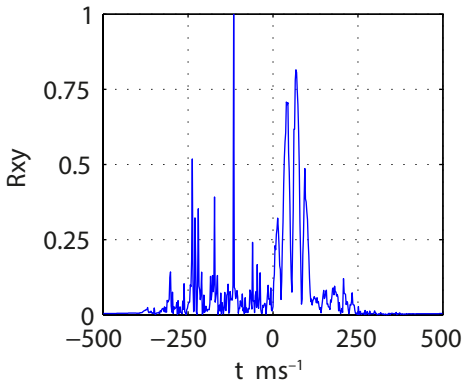
(h) GCC, GSNR = 15 dB
