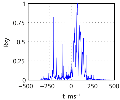
(j) PHAT-GCC, GSNR = 15 dB
