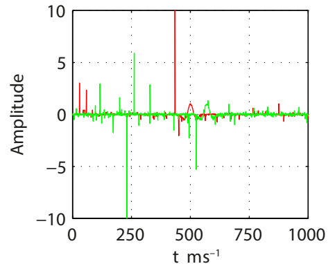
(f) PHAT-GCC, GSNR = 0 dB
