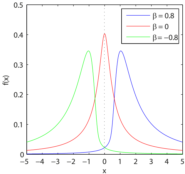
(a) \alpha -stable densities, \alpha = 0.7, \gamma = 1, \delta = 0
