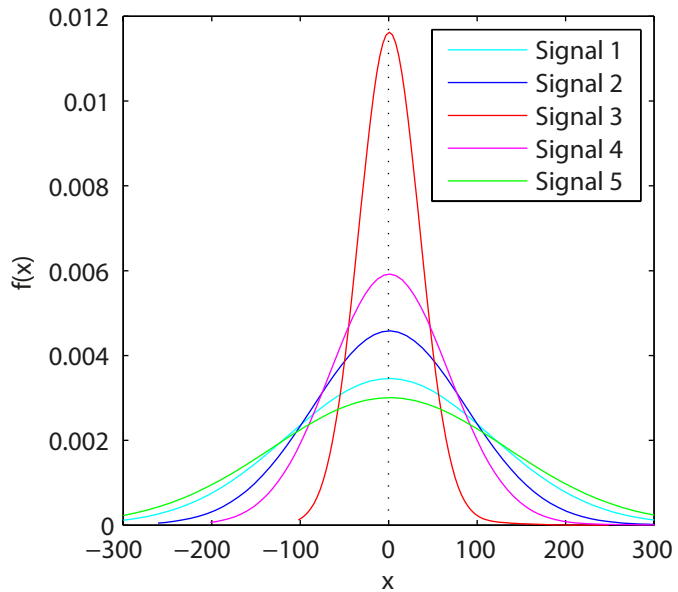
(b) \alpha -stable densities of micro-seismic signals
