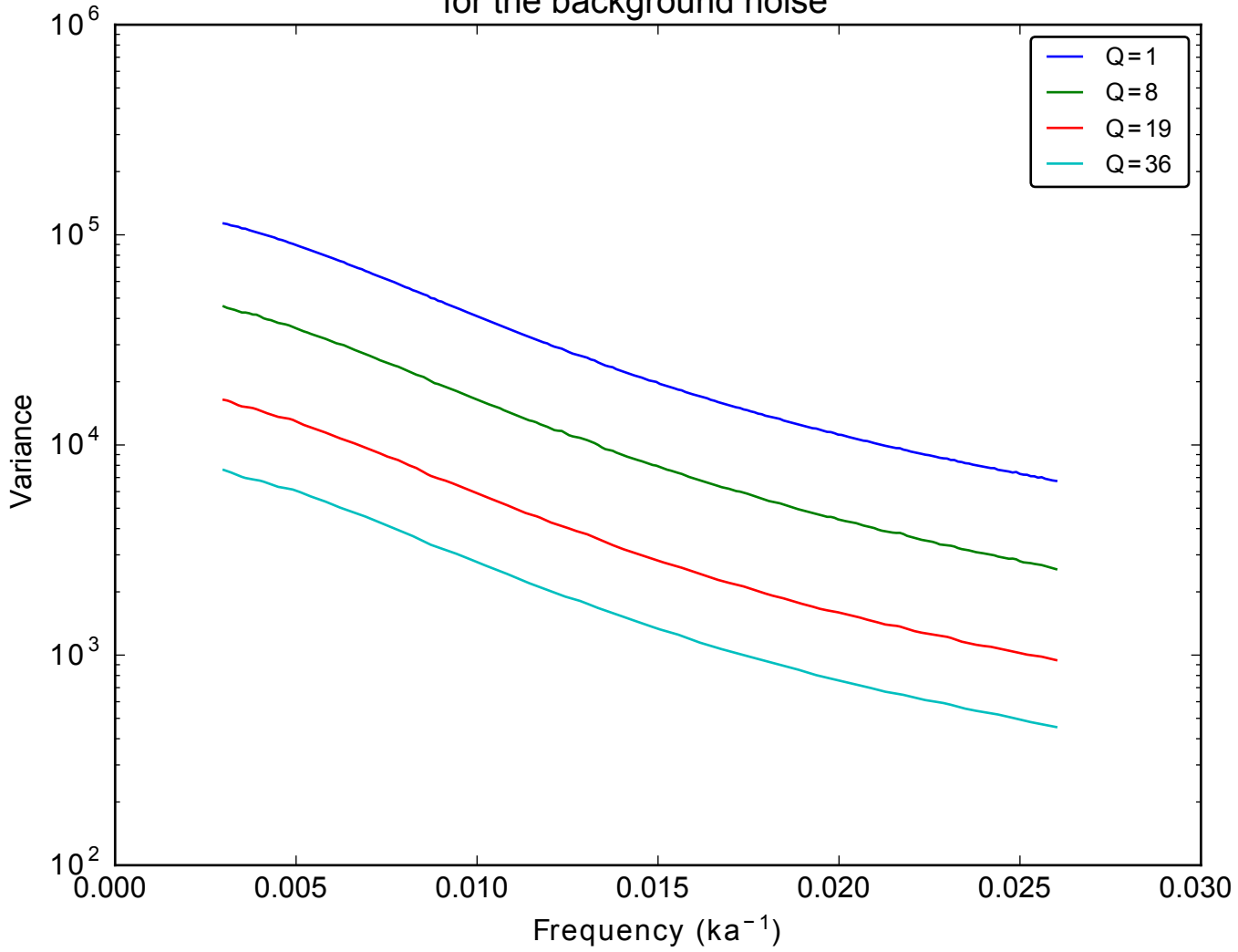
Analytical variance of the WOSA periodogram for the background noise
