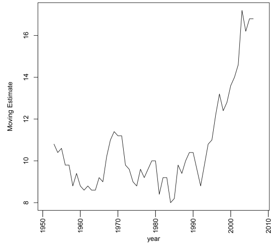
Figure 3. A moving average estimate of the average number of tropical storms between 1951 and 2008.
