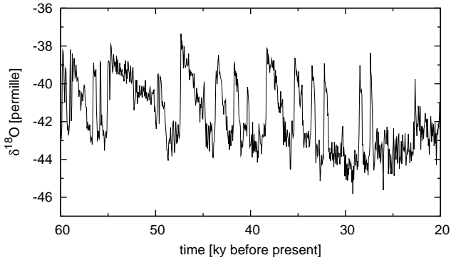
Fig. 4. Record of \delta^{18}\text{O} from the NGRIP ice core for the last glacial period.
