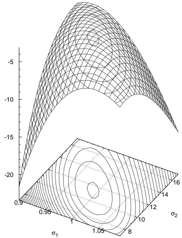
Fig. 2. Simulated data: Log-likelihood as a function of the noise levels \sigma_1 and \sigma_2 . Neighbouring contours differ by a factor of 2 in likelihood.
