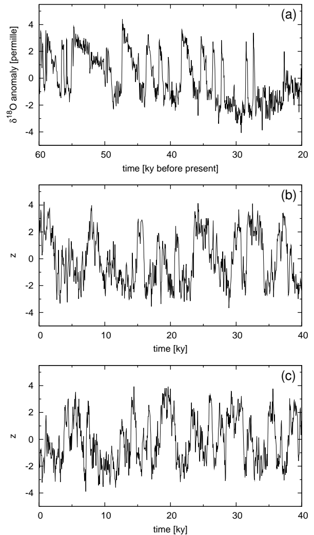
Fig. 8. (a) Record of \delta^{18}\text{O} from the NGRIP ice core for the last glacial period with the mean value removed. (b) Sample trajectory of the oscillator model. (c) Sample trajectory of the one-dimensional potential model.
