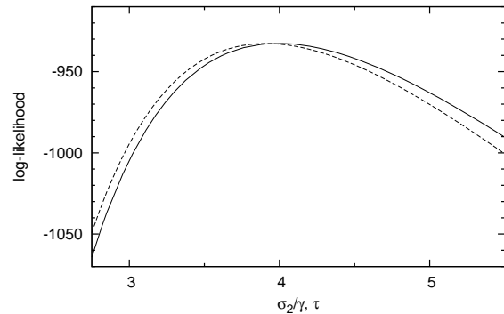
Fig. 6. Ice-core data: Log-likelihood as a function of \sigma_2/\gamma for the oscillator model (solid) and as a function of \tau for the one-dimensional potential model (dashed).
