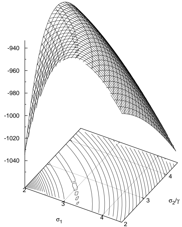
Fig. 5. Ice-core data: Log-likelihood as a function of the noise levels \sigma_1 and \sigma_2 . Neighbouring contours differ by a factor of 100 in likelihood.
