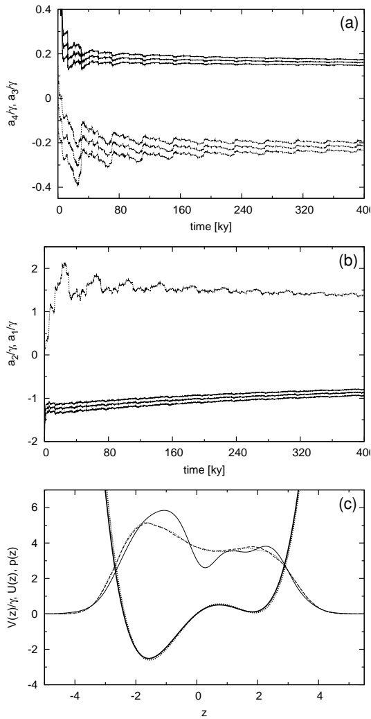
Fig. 7. Ice-core data: (a) Estimates for a_4/\gamma and a_3/\gamma with error standard deviation. (b) Estimates for a_2/\gamma with error standard deviation and estimates for a_1/\gamma . (c) Scaled potential V(z)/\gamma for the oscillator model (thick solid) and potential U(z) for the one-dimensional model (thick dotted). Probability densities of the ice-core data (solid), the oscillator model (dotted) and the one-dimensional model (dashed).
