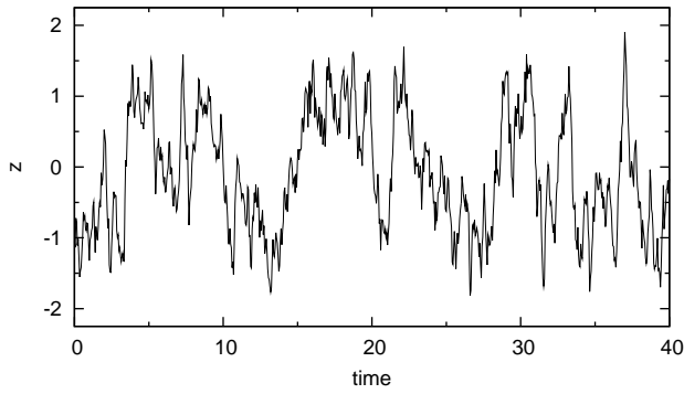
Fig. 1. Sample trajectory of z in the oscillator with symmetric double-well potential.
