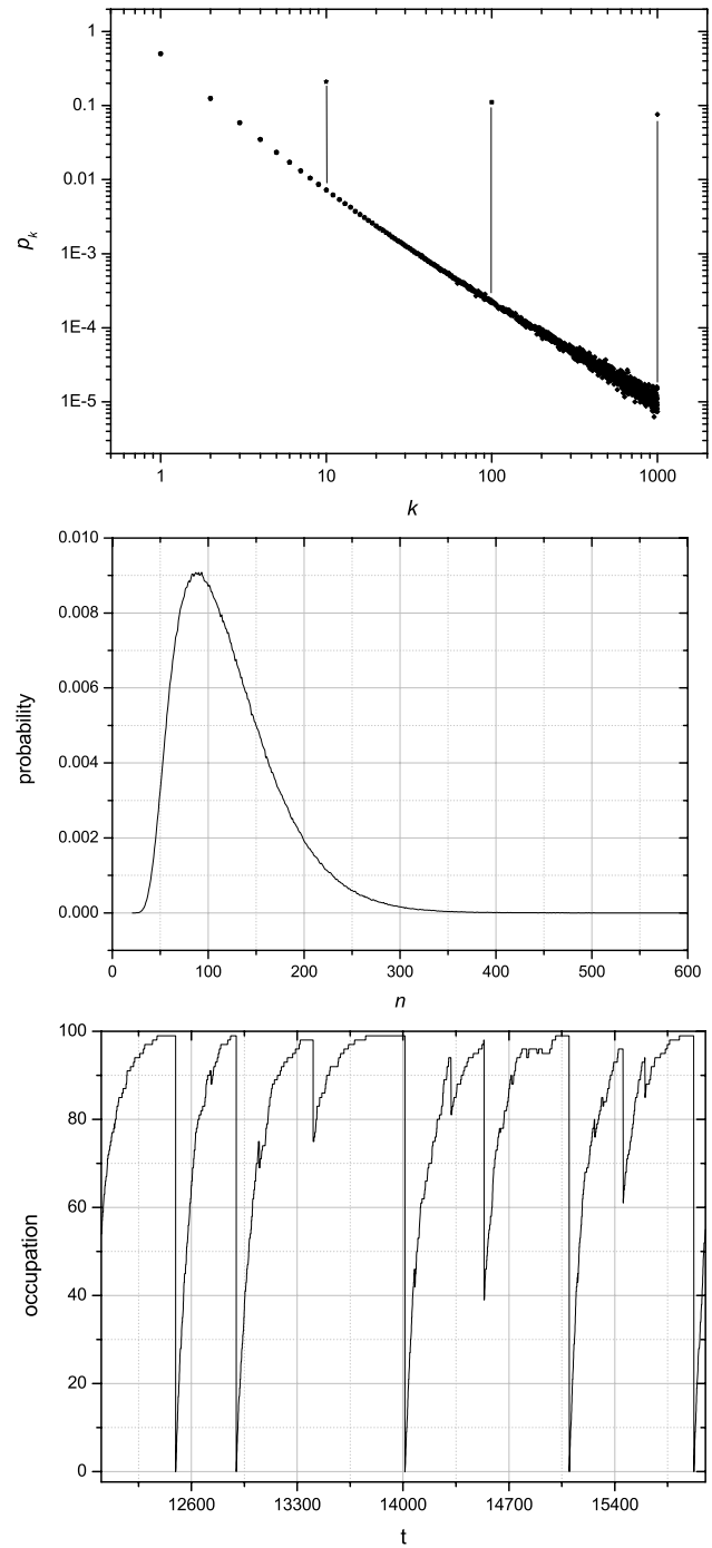
Fig. 1. (a) Probability of occurrence of earthquakes of size k . Note that the simulations corresponding to N equal to 10, 100, and 1000 are superimposed. (b) For N = 20 , the probability of return of the characteristic earthquake as a function of the time elapsed since the last event, n . (c) Time evolution of the state of occupation in a system of size N = 100 . Note that after each characteristic event that completely depletes the system, there follows the corresponding recovery up to a high level of occupancy, and then the system typically presents a plateau previous to the next characteristic earthquake.
