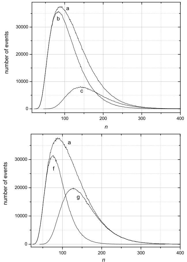
Fig. 3. (a) For N = 20 . Line a is the distribution of return times of the characteristic earthquake as a function of the time elapsed since the last event, n . Line b corresponds to the distribution of cycles where no medium-size earthquake occurs. Line c corresponds to cycles with medium-size earthquakes. Curves b and c constitute the splitting of curve a according to whether this retarding effect is fulfilled or not. (b) Lines f and g , represent the separation of the a distribution according to whether the advancing effect is fulfilled or not.
