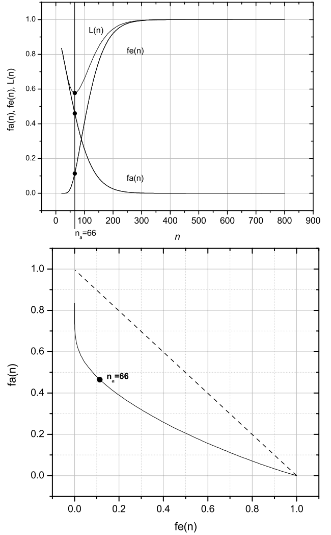
Fig. 2. For N = 20 , (a) Fraction of failures to predict, f_e , fraction of alarm time, f_a , and loss function L = f_a + f_e as a function of n . (b) Error diagram for characteristic event forecasts based on n . The diagonal line would correspond to a random strategy.
