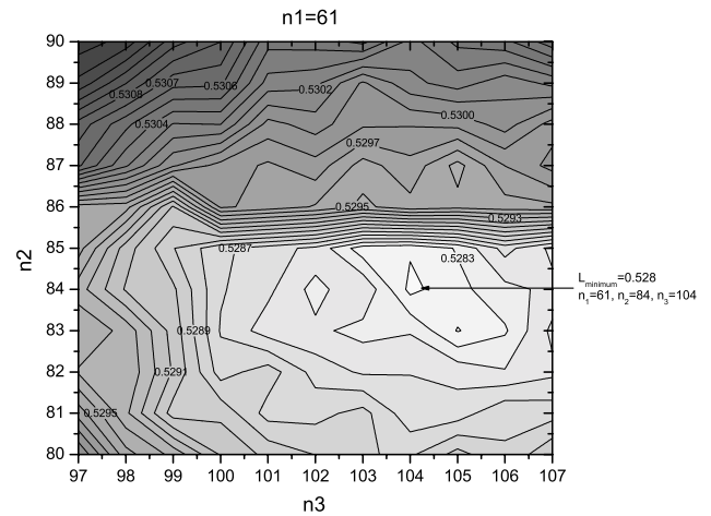
Fig. 5. For N = 20 . Illustration of the three-dimensional strategy. For n_1 = 61 , L -constant level-curves are plotted. The minimum value of L is 0.528 for n_1 = 61 , n_2 = 84 , n_3 = 104 .
