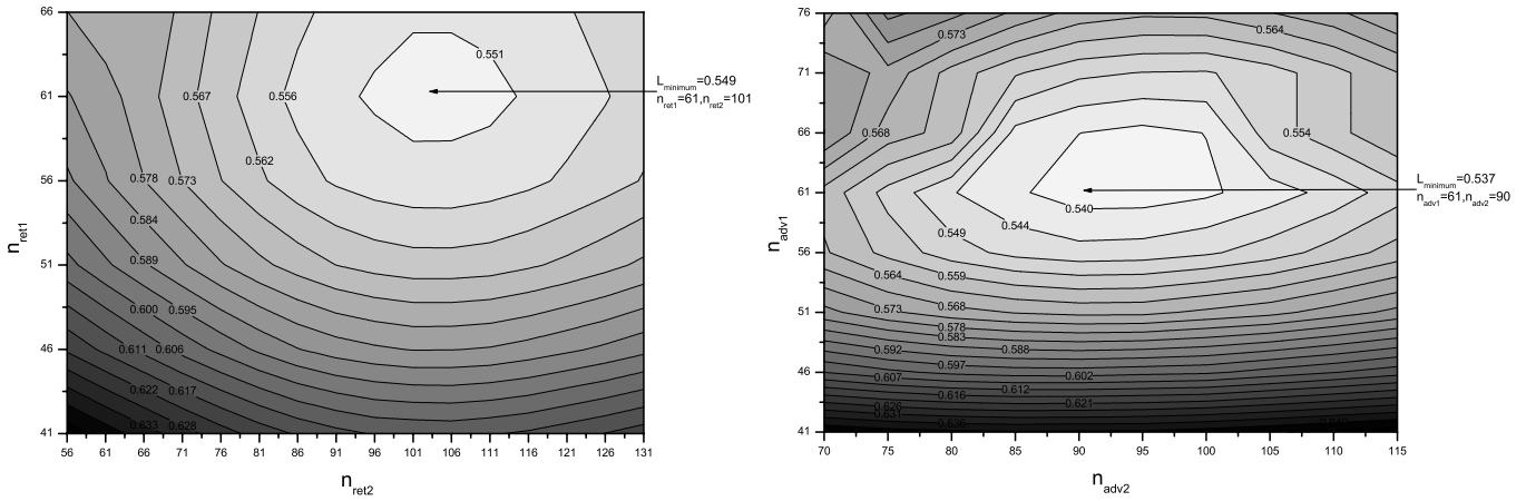
Fig. 4. (a) For N = 20 . Results of the two-dimensional strategy based on the splitting of curve a according to whether the retarding effect is fulfilled or not. Values of L varying n_{ret1} and n_{ret2} . Minimum value of L = 0.549 for n_{ret1} = 61 and n_{ret2} = 101 . (b) Results of the two-dimensional strategy based on the splitting of curve a according to whether the advancing effect is fulfilled or not. Values of L varying n_{adv1} and n_{adv2} . Minimum value of L = 0.537 for n_{adv1} = 61 and n_{adv2} = 90 .
